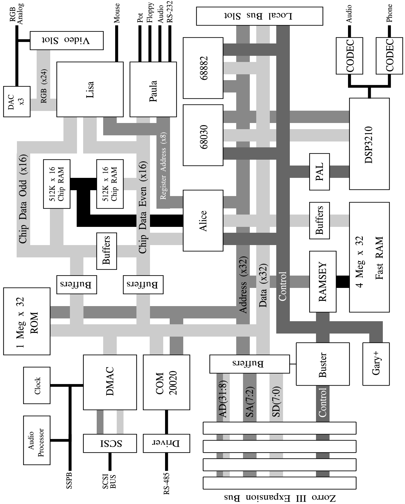
Figure 1-1: Amiga 3000+ System Structure
